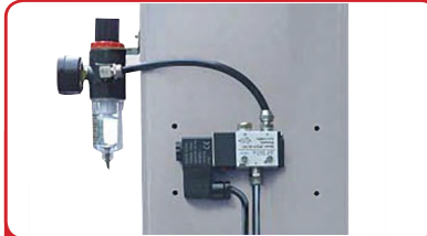
Oil-water separator and Solenoid air valve installed outside the control box
